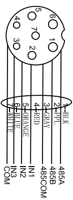
CONTROL PORT (7 pins)
